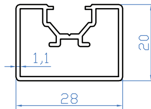
K2227 DEKOR (0.345 Kg/m)
