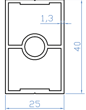
K2208 25X40 DİKME (0.650 Kg/m)
